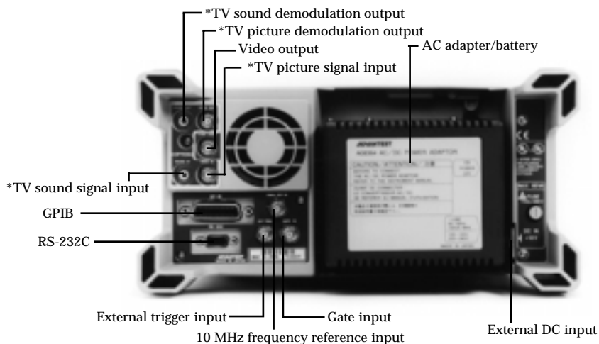
Rear panel
