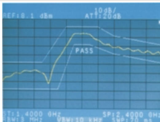
PASS/FAIL evaluation using upper and lower limit line
